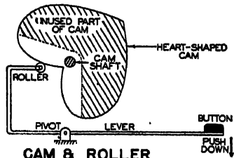
CAM & ROLLER
